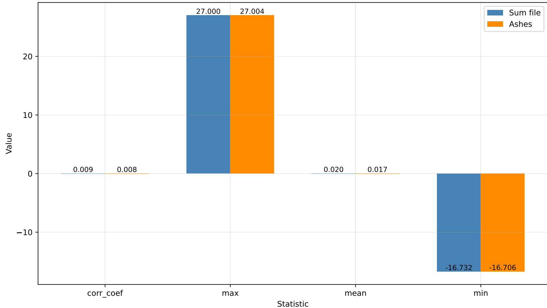
v'w' Reynolds Stress Comparison
