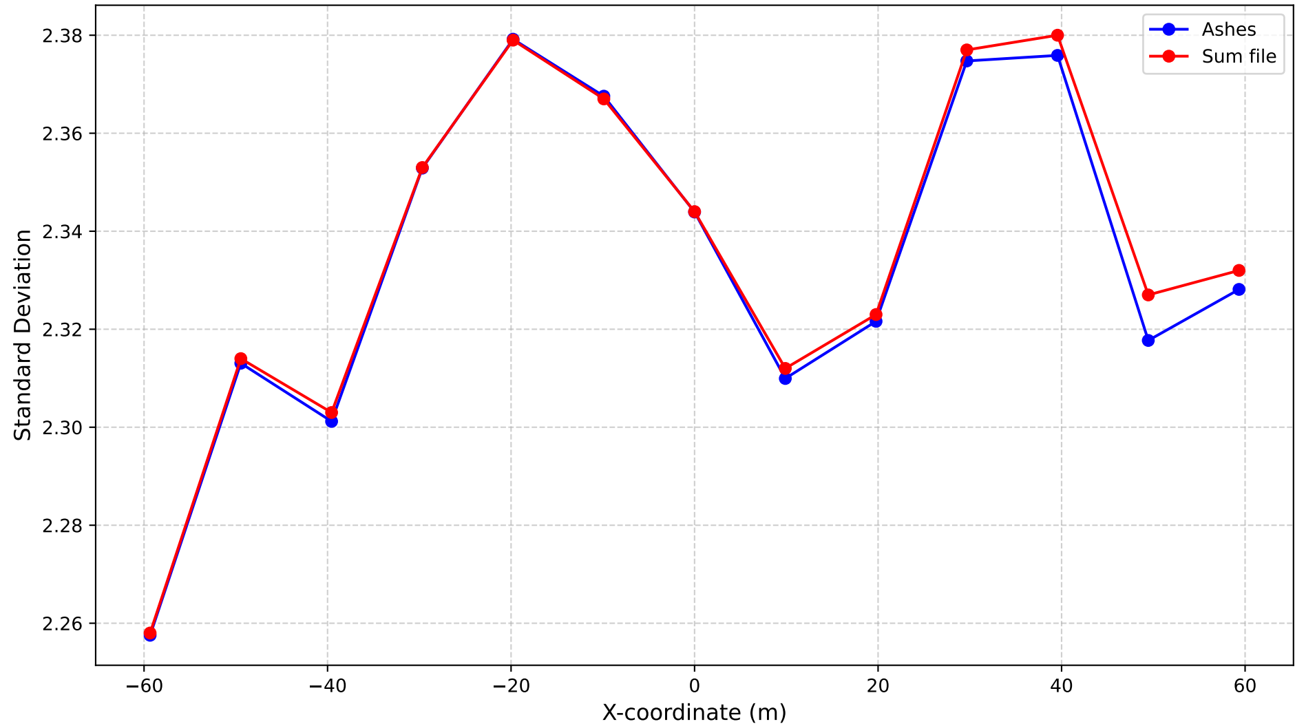
U Component Standard Deviation at Height 112.8 m
