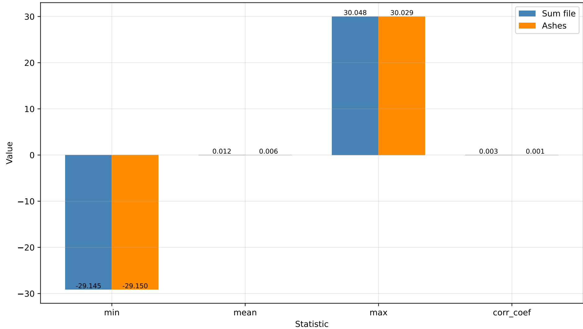
Reynolds u'v' Comparison
