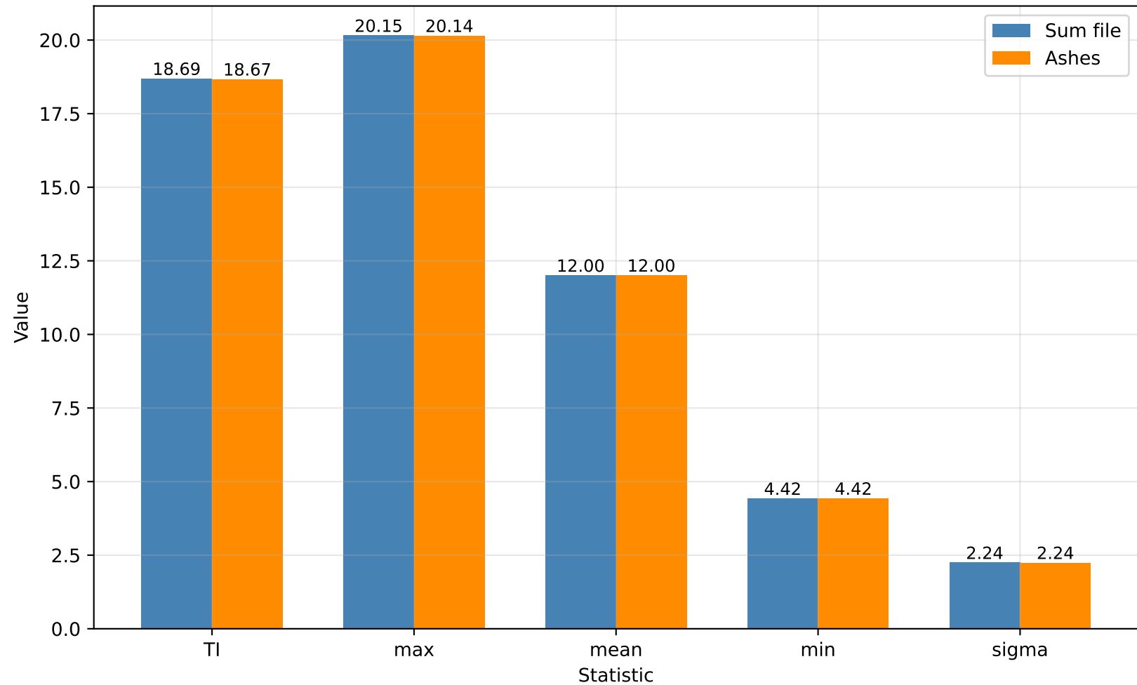
u Component Statistics Comparison
