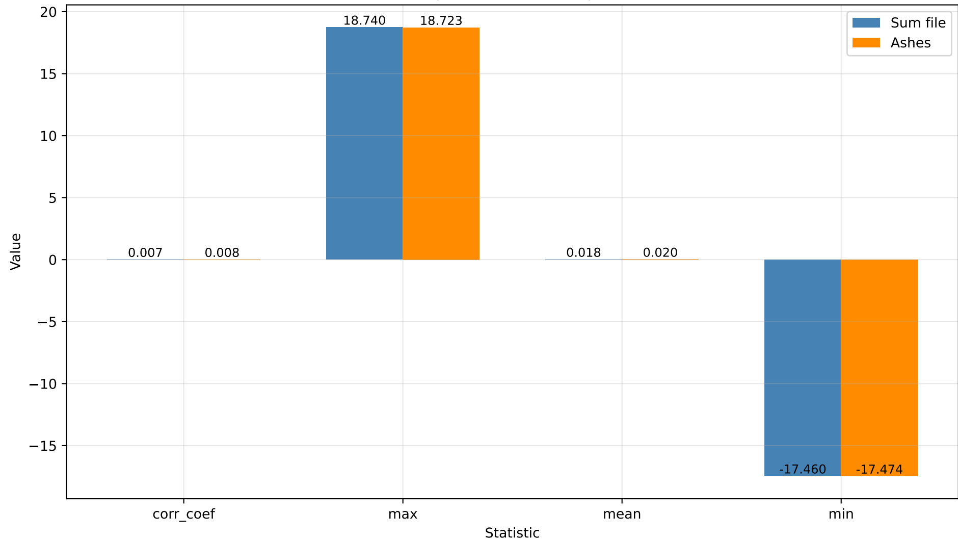
u'w' Reynolds Stress Comparison
