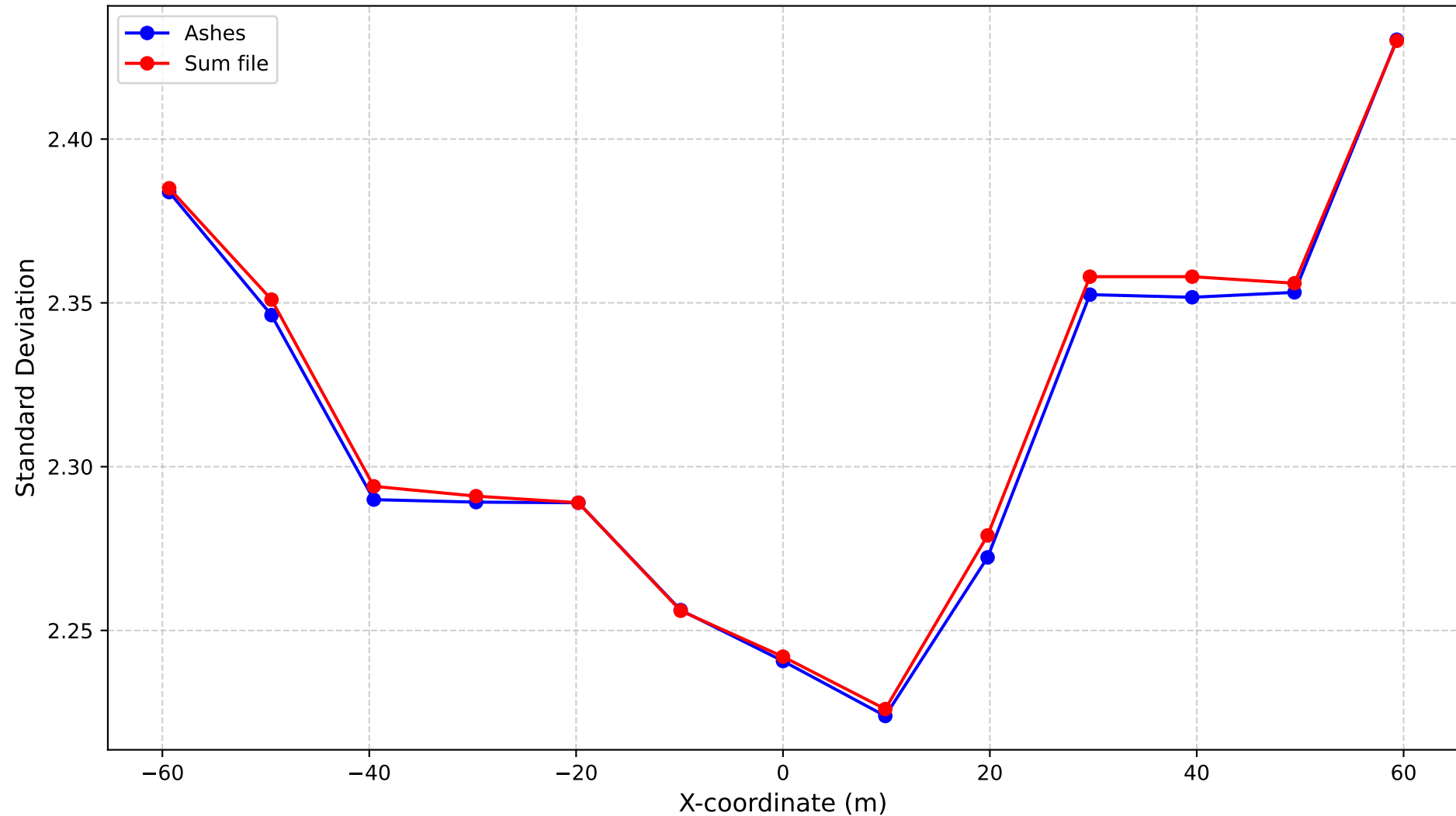
U Component Standard Deviation at Height 152.4 m
