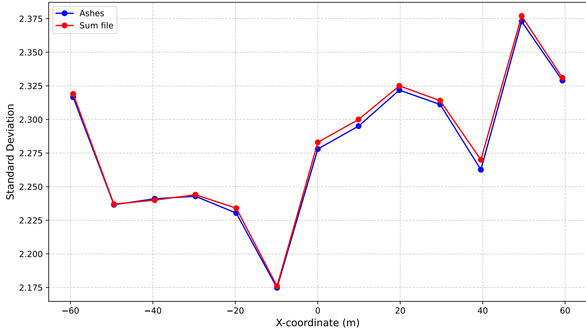
U Component Standard Deviation at Height 192.0 m
